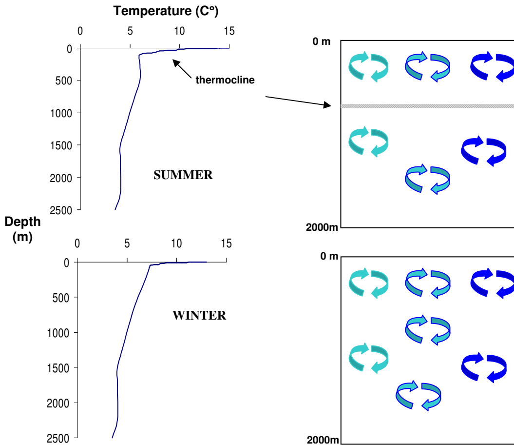
Figure 1: The temperature of ocean water over summer and winter at different depths and a diagram showing the mixing of water in the different water layers.
